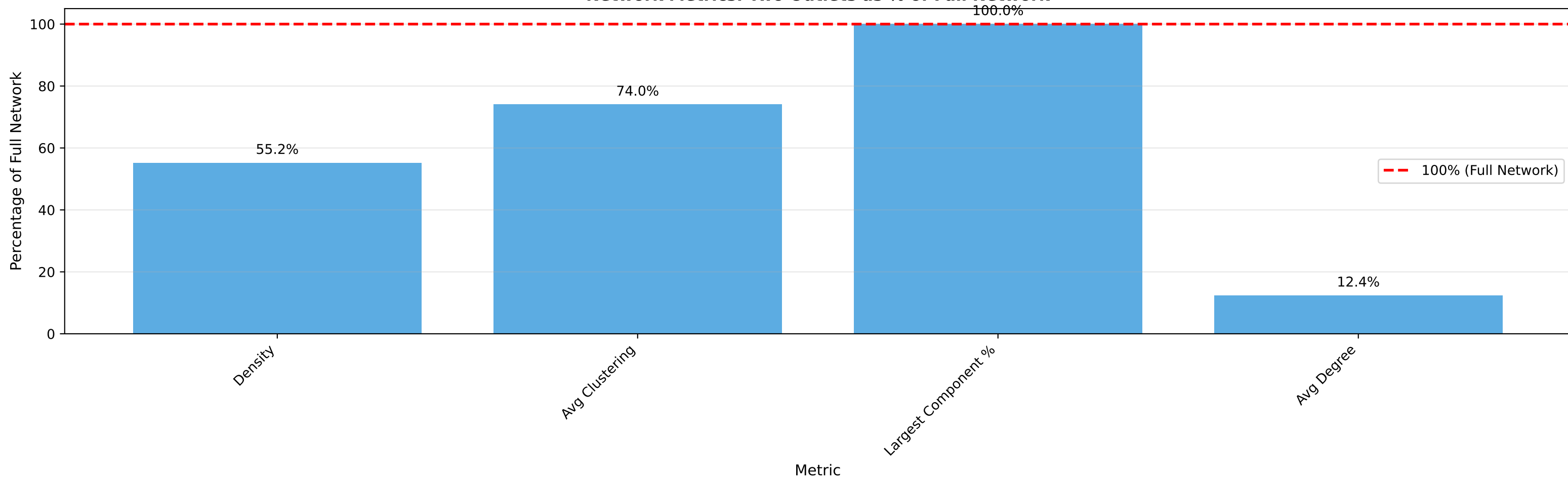
Network Metrics: Two Outlets as % of Full Network
